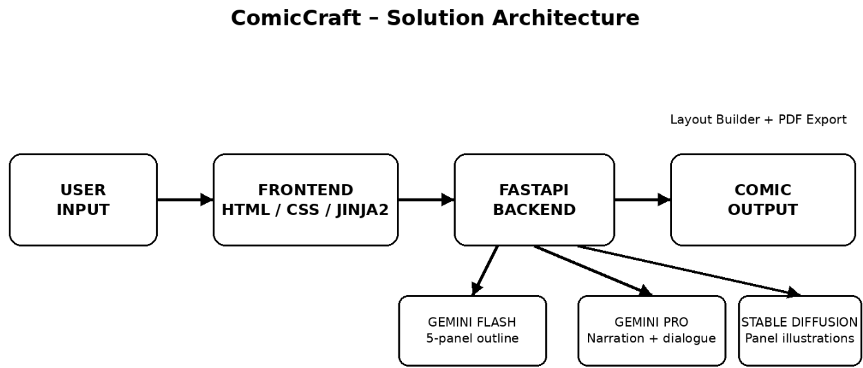
Figure: Architecture and data flow of the ComicCraft AI comic generation application
